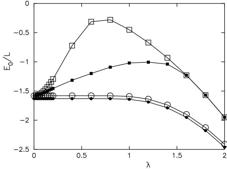
Fig.1. Numerical results for upper and lower bounds to the ground state energy per site E_0/L of the two-dimensional Holstein model as a function of the EP coupling \lambda . Open squares: Variational results using the BCS trial Hamiltonian with a fixed oscillator frequency. Solid squares: Variational results using the BCS trial Hamiltonian and an adjustable oscillator frequency. Circles: Upperbounds as obtained from a simulated-anneal minimization of the r.h.s. of (30) for a lattice of 12 \times 10 sites. Bullets: Lowerbounds as obtained from a simulated-anneal minimization of the l.h.s. of (23) for a lattice of 12 \times 10 sites. In all cases the density of electrons \langle n \rangle = 1 .
