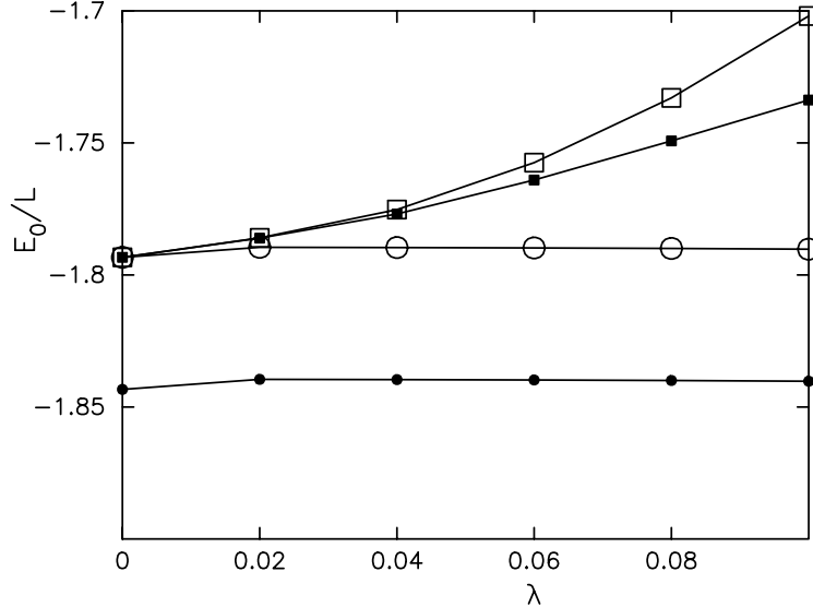
Fig.3. Same as Fig.1 except that \langle n \rangle = 1.383 .
