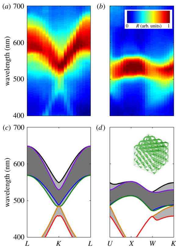
Figure 4. Photonic band structure diagrams (PBSDs). Measured ( a,b ) and simulated ( c,d ) PBSDs for a single-network diamond-type photonic crystal ( Fd3m ) along the paths ( a,c ) L-K-L and ( b,d ) U-X-W-K , respectively. The grey areas in ( c,d ) indicate the photonic bandgap of the investigated structure, corresponding to the measured reflectance bands in ( a,b ). In the simulation, the dielectric constant was \epsilon = 2.45 and the chitin filling fraction was approximately 0.3 ( t = -0.5 ). For the wavelength conversion in ( c,d ), the cubic lattice constant of the photonic crystal was set to a = 445 nm (see also electronic supplementary material, figure S4). The inset shows a rendered model of the single diamond photonic crystal.
