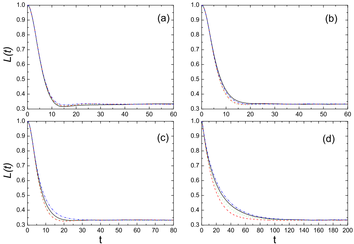
FIG. 5. (Color online) The time evolution of the Loschmidt echo L(t) of a central system (with J=-5 ), which interacts with a Heisenberg-type environment H_e via a Heisenberg ( \Delta=-0.075 ) Hamiltonian H_{ce} . In each panel, the values of \sqrt{K}\Omega are the same: (a) \sqrt{K}\Omega \equiv 0.1\sqrt{N-1} , (b) \sqrt{K}\Omega \equiv 0.15\sqrt{N-1} , (c) \sqrt{K}\Omega \equiv 0.25\sqrt{N-1} , and (d) \sqrt{K}\Omega \equiv \sqrt{N-1} . The different lines in each panel correspond to different K . Solid (black) line: K=2 ; dashed (red) line: K=4 ; dotted (green) line: K=6 ; and dash-dotted (blue) line: K=N-1 .
