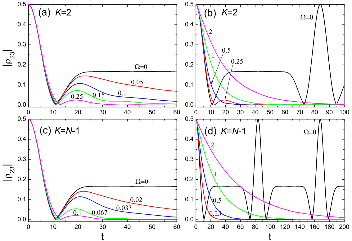
FIG. 2. (Color online) The time evolution of the off-diagonal element \rho_{23} of the reduced density matrix of a central system (with J=-5 ), which interacts with a Heisenberg-type environment H_e via an isotropic Heisenberg Hamiltonian H_{ce} (with \Delta=-0.075 ) for the same geometric structures in the environment: [(a) and (b)] K=2 and [(c) and (d)] K=N-1 . The number next to each curve is the corresponding value of \Omega .
