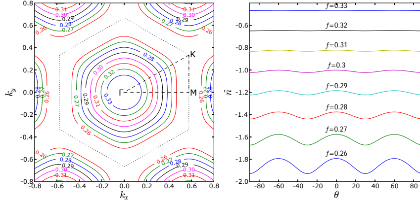
Fig. 1. Left: Equifrequency surface plot of TM modes for a triangular lattice photonic crystal consisting of air holes with a radius of r = 0.4a , drilled in a dielectric medium ( \epsilon = 12.96 , \mu = 1 ) for the frequency range f = 0.26 - 0.33 . The first Brillouin zone of a triangular lattice (dotted line) and the symmetry points are also shown. Right: Effective refractive index \hat{n} as a function of the angle \theta of the incoming wave vector \mathbf{k} for the frequency range f = 0.26 - 0.33 .
