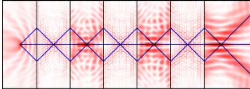
Fig. 4. Same as the left panel of Fig. 2 for a cascaded stack with three PhC slabs. For the description of the imaging system we refer to the text.
