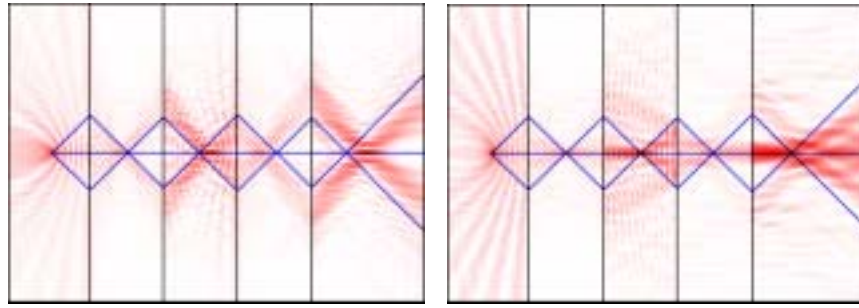
Fig. 3. Same as the left panel of Fig. 2 for f = 0.300 (left) and for air/PhC interfaces that are not cut (right).
