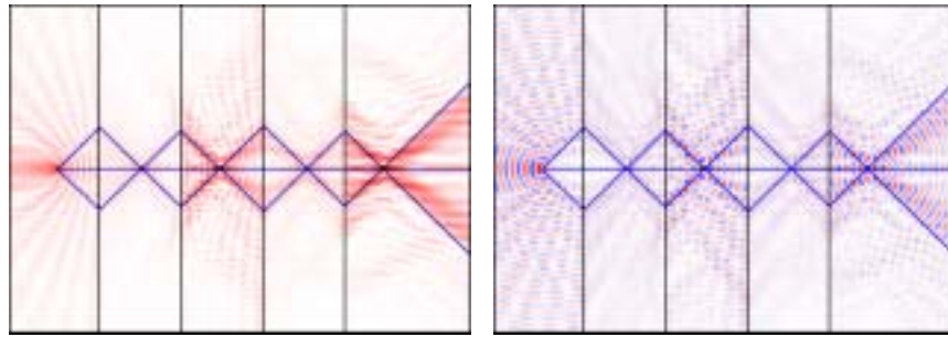
Fig. 2. Left: Intensity of the electric field of a TM wave with frequency f = 0.299 , generated by a point source placed in front of a cascaded stack composed of two PhC slabs with an air layer in between. For the description of the imaging system we refer to the text. The blue lines indicate the propagation directions according to Snell's law for a homogeneous slab with \hat{n} = -1 . Intensities are plotted on a \log_{10} scale. The field intensities are scaled between 0 and 1. Because the transmitted intensity is low, the intensities are scaled different for the regions to the left of the stack, in between the slabs, behind the stack and inside the slabs. Right: Amplitude of the electric field. The electric field amplitudes are plotted on a linear scale ranging from -1 to +1 (blue: Negative values, red: Positive values) and are scaled different for the regions to the left of the stack, in between the slabs, behind the stack and inside the slabs.
